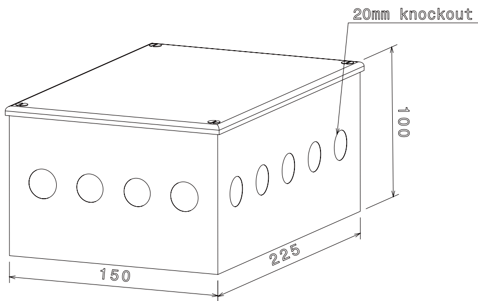
Isometric view
