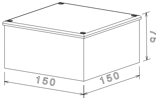
Isometric view
