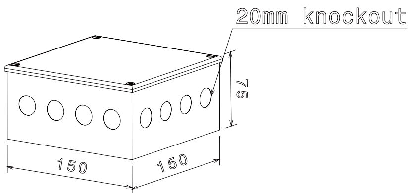
Isometric view
