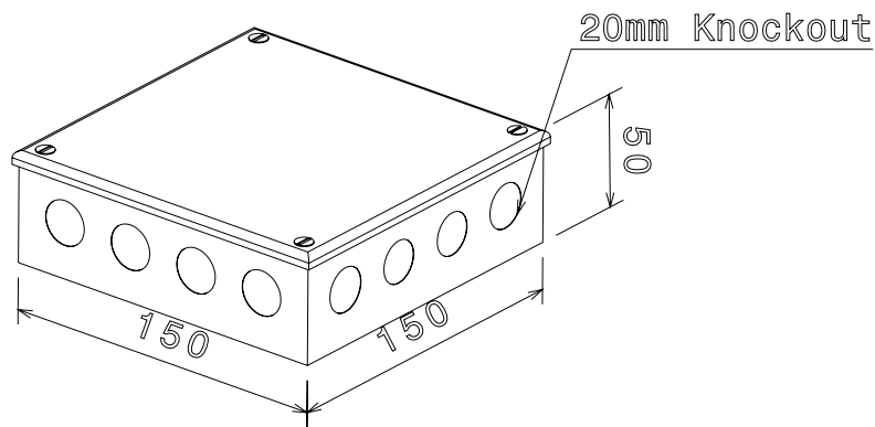
Isometric view
