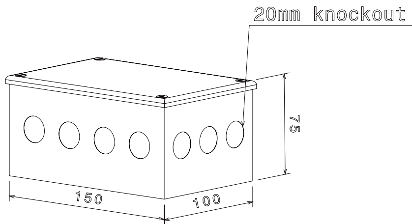
Isometric view
