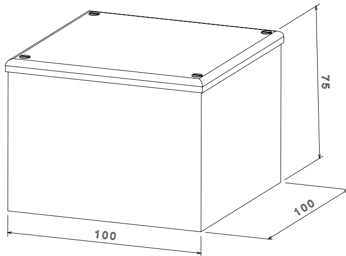
Isometric view
