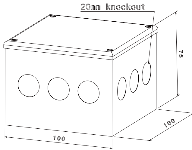
Isometric view
