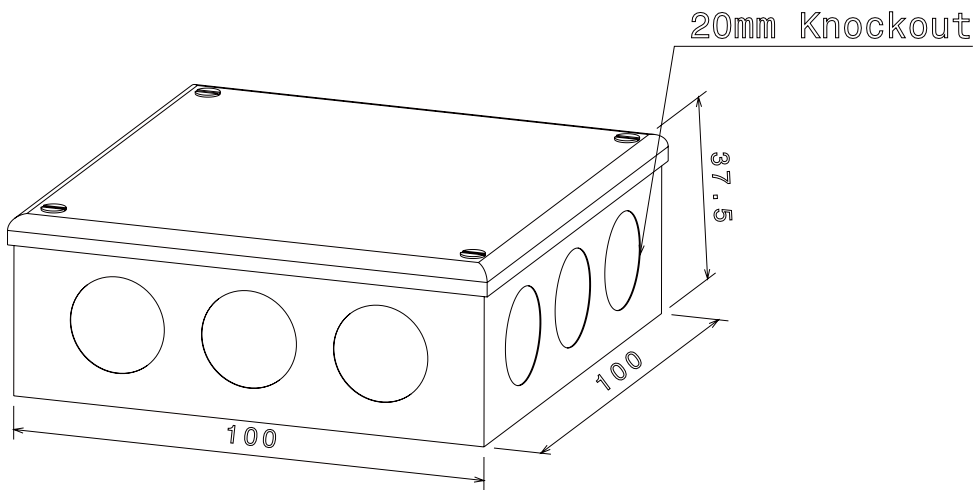
Isometric view
