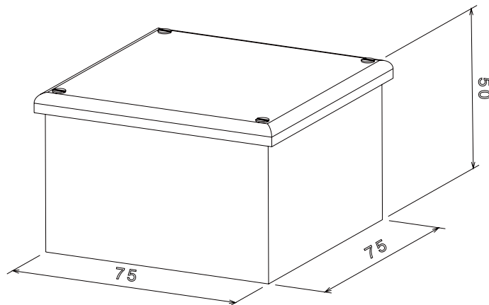
Isometric view
