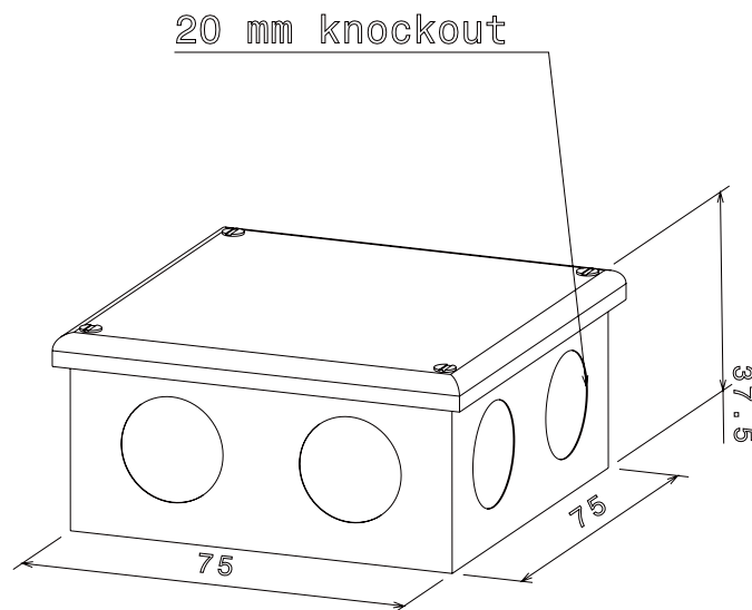
Isometric view
